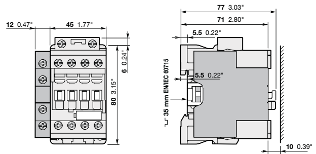
NF.22E, NF.31E, NF.40E + CAL4-11 2-poliger Hilfskontaktblock
